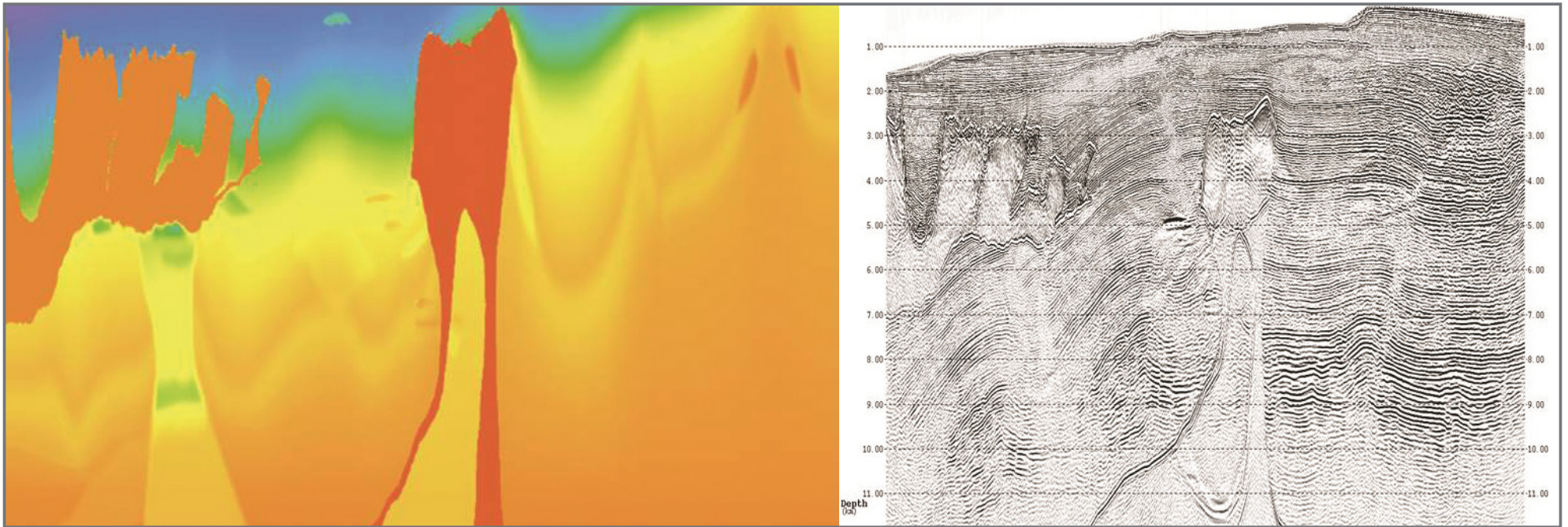
BP 2004 salt model and Aspen Echos RTM image.
