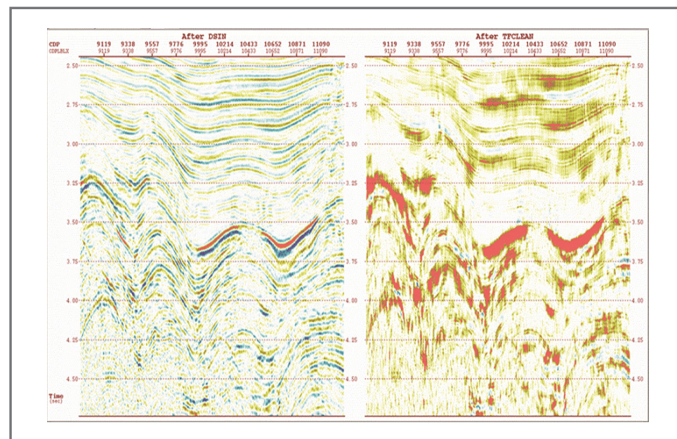
Aspen Echos seismic data analysis with relative permeability extractions.
